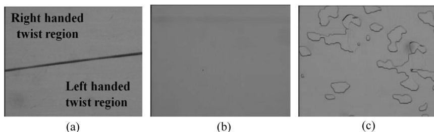
FIGURE 3 The alignment textures of the sample with different injection temperature at (a) 50^{\circ}\text{C} , (b) 103^{\circ}\text{C} \sim 113^{\circ}\text{C} , and (c) 130^{\circ}\text{C} .
