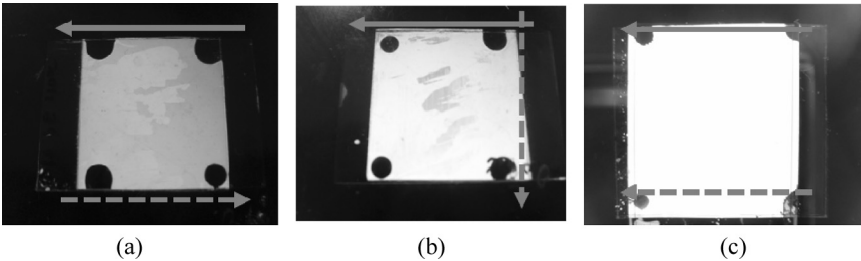
FIGURE 4 The textures of samples under crossed polarizers with different direction of LC injection with respect to the rubbing direction. The solid and dotted lines indicate LC injection and rubbing direction, respectively.
