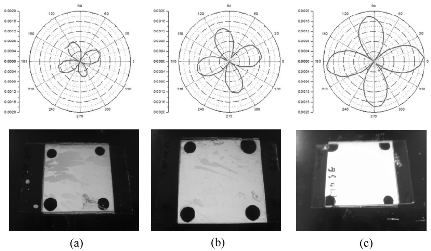
FIGURE 5 The birefringence of polyimide layer and the alignment textures with different number of rubbing; (a) 1 time, (b) 5 times, and (c) 10 times.
