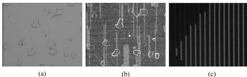
FIGURE 2 The microscopic images of CH-IPS sample; (a) without field, (b) with intermediate, and (c) with high field.
