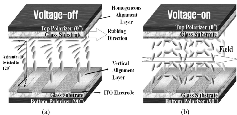
FIGURE 1 Schematic diagrams of CH-IPS mode in bright and dark state.
